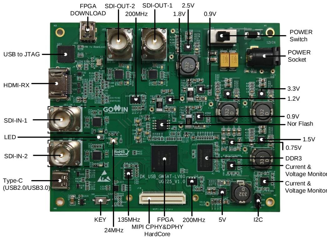
Figure 2-3 PCB Components
